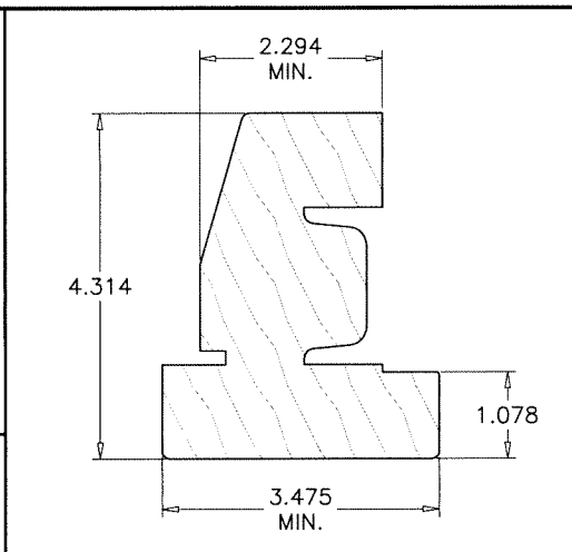
4 OUTSWING SIDE STILE
