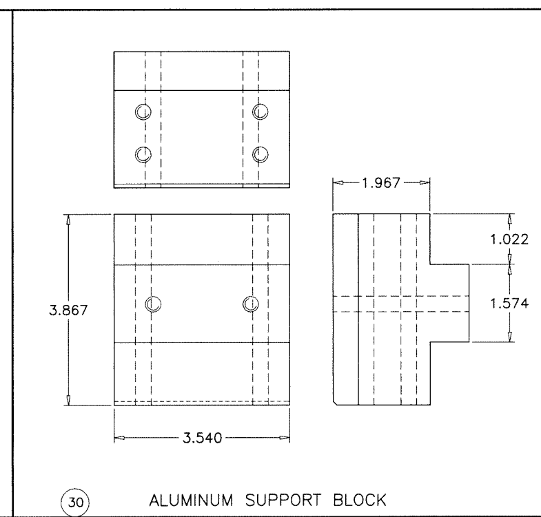
SUPPORT BLOCK DETAIL AT SILL
