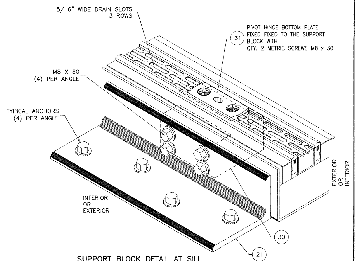
SUPPORT BLOCK DETAIL AT SILL
