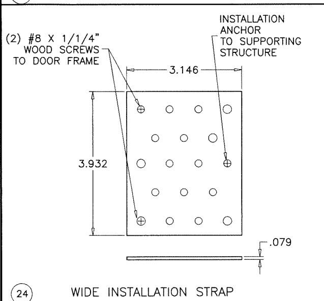
(23) NARROW INSTALLATION STRAP
